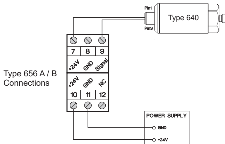
Type 656 A / B connected to Vibration Control Type 640 and Power Supply
